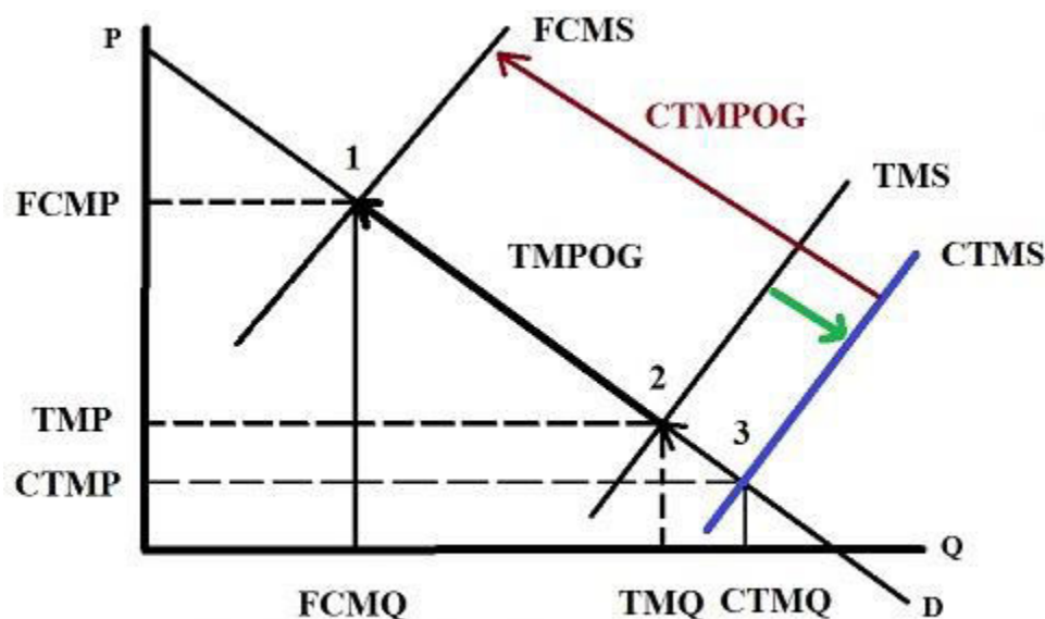
Figure 5 The full cost pricing-Circular traditional market pricing framework
