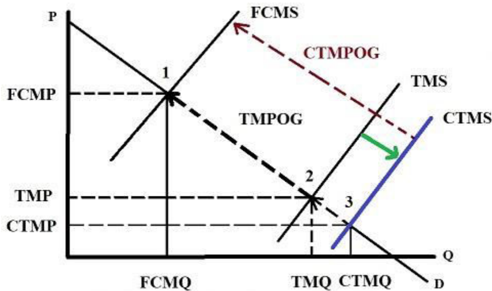
Figure 7 The full cost pricing-EU inspired circular traditional market pricing framework Under pareto optimality gap neutrality assumptions
